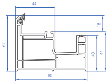
Monorail Sliding Frame 3104-1104
