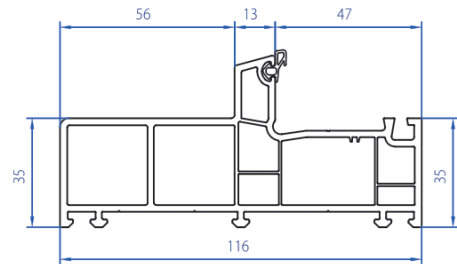
Frame with Grill & Mesh 2101-1102
