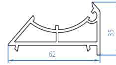
Bay Pole Adaptor 2108-3104
