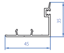
Sliding Window Interlock 2106-3101
