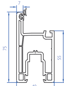
Sliding Sash 2105-1102
