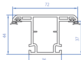
Sliding Mullion 3102-1104
