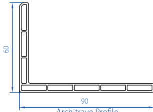
Architrave Profile 2108-3102
