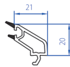
Sliding Single Glazing Bead (5-6mm) 2107-4101
