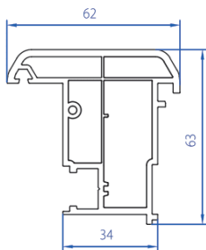
French Mullion 2102-1103
