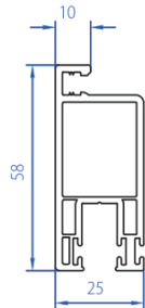
Fly Mesh Sash (Big) 2105-3105
