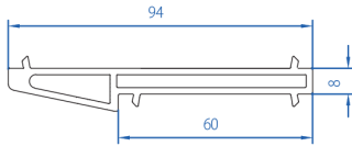
Casement-Sliding Profile Coupler (PRIMA) 50502-11039
