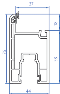
Sliding Sash 3105-1102
