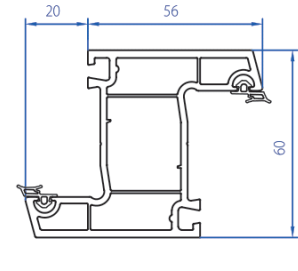
Z-Mullion 2102-1102
