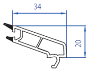
Casement Glazing Bead (5-6mm) 2107-4103
