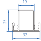
Fly Mesh Sash (Big) Mullion 50502-11058
