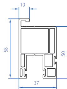
Fly Mesh Sash (For 3 Track) 2105-3106
