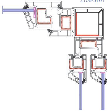
90° Corner Coupling 2108-3101
