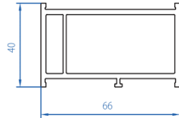
Coupling/ Extension Profile 2108-3106
