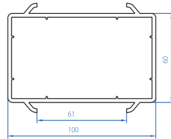
Heavy Duty Coupling 2108-3109
