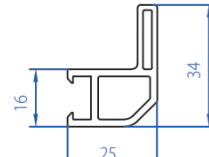
Clip On Frame 4104-3102
