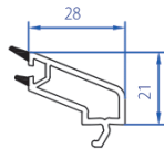
Casement Glazing Bead (12mm) 2107-4104
