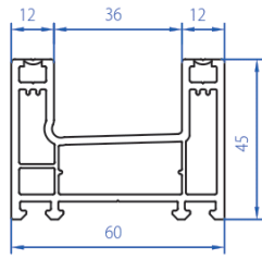
2T Sliding Frame 2104-3101
