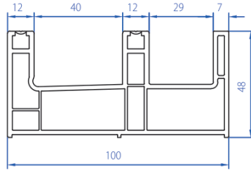
Sliding Frame with Mesh 3104-3103
