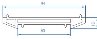
Casement-Sliding Profile Middle Coupler (PRIMA) 50502-11040
