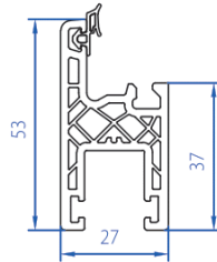
Eco Sliding Sash 4105-1101
