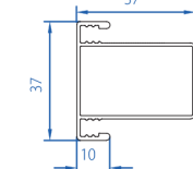
Super Screen Sash Mullion-3T 50502-11077
