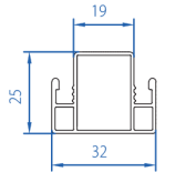
Fly Mesh Sash (Small) Mullion 50502-11037
