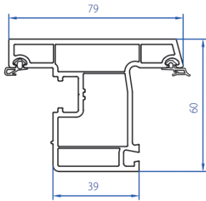
Outward Window Sash 2103-1101
