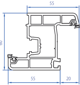
Inward Window Sash 2103-1103
