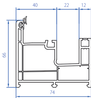
Monorail Sliding Frame 2104-1104
