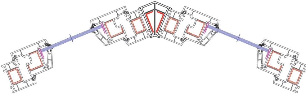
135° Corner Coupling 2108-3110
