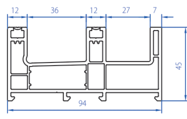
Sliding Frame with Mesh 2104-3103
