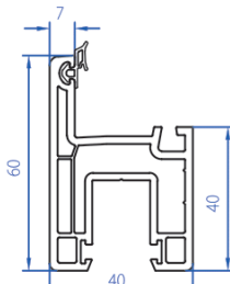
Sliding Window Sash (Non-Euro groove) 2105-1101
