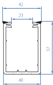
Stiffener Profile 2108-4107
