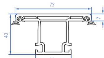
Sliding Mullion 2102-1104
