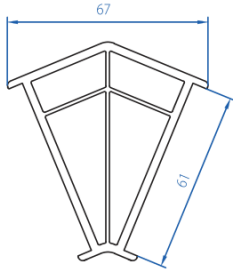
135° Corner Coupling 2108-3110
