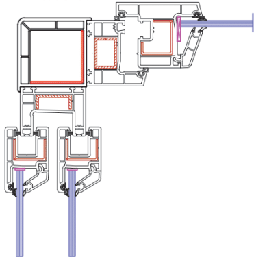
90° Corner Coupling 2108-3101
