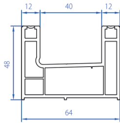
2T Sliding Frame 3104-3101
