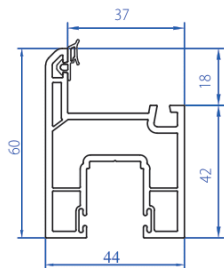
Sliding Window Sash (Non-Euro groove) 3105-1101
