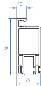
Fly Mesh Sash (Big) 2105-3105
