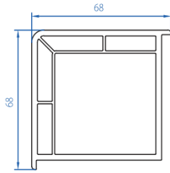
90° Corner Coupling 2108-3101
